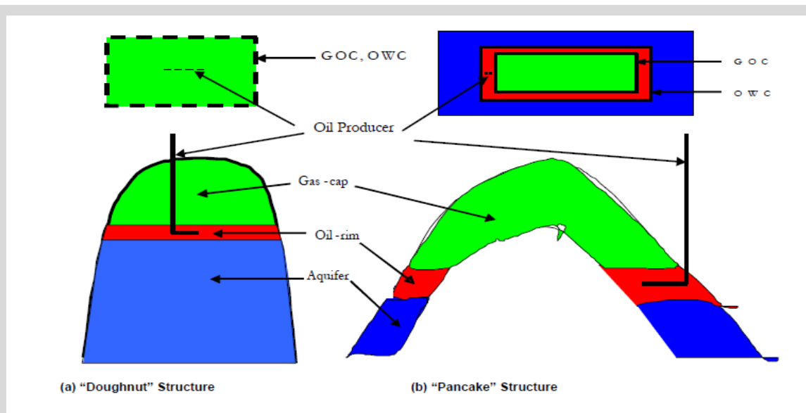
Figure 7: A typical model of an oil rim reservoir ( Lawal et al., 2010)
